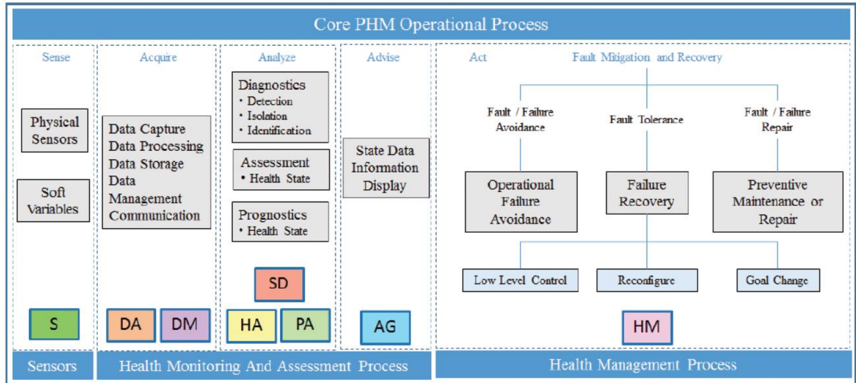
Figure A.2—PHM system operational view
